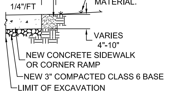
SECTION WHERE CONCRETE ADJOINS LANDSCAPING
