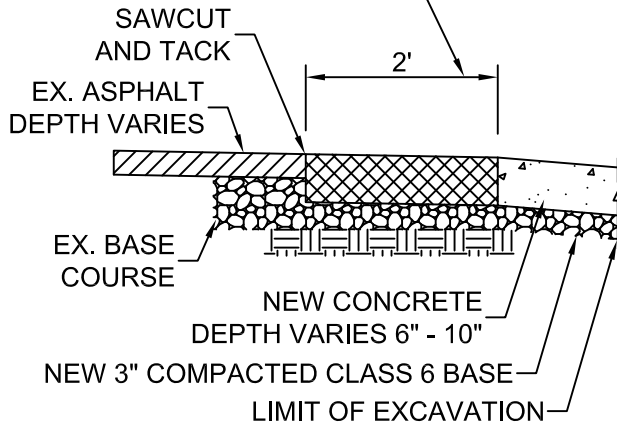
SECTION WHERE CONCRETE ADJOINS ASPHALT
